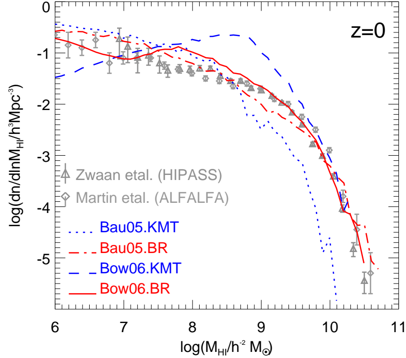
Figure 4.6: The HI mass function at z = 0 for the Bau05.KMT (dotted line), Bau05.BR (dot-dashed line), Bow06.KMT (dashed line) and Bow06.BR (solid line) models. Symbols show the z = 0 observational estimates from Zwaan et al. (2005) using HIPASS and from Martin et al. (2010) using ALFALFA, as labelled.
